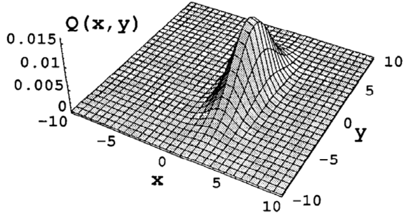
Fig. 4.1 Q function for a squeezed state with coherent amplitude \alpha = 2.0 , r = 1.0
